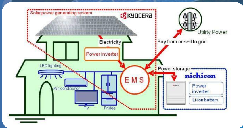
Solar System Example
